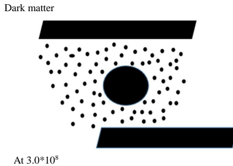
Fig. 1: “Dark matter” at the speed of light. Wave undergoing gravitational lensing
