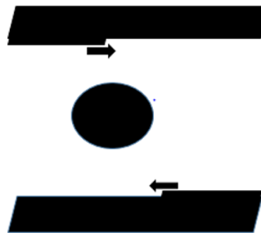
Fig. 2: Gravitational mechanism
