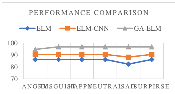
Fig. 4: Accuracy performance comparison
