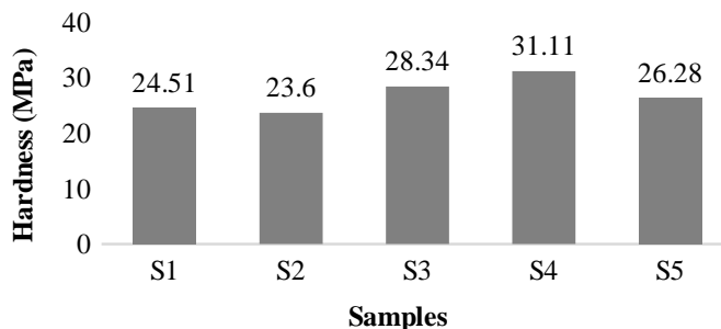
Fig. 6: Hardness test results
