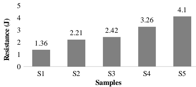
Fig. 4: Results of Impact Test (J)
