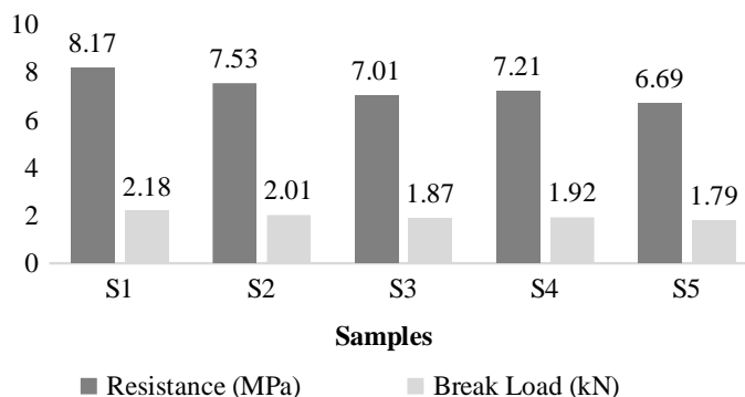
Fig. 7: Results of the flexion test
