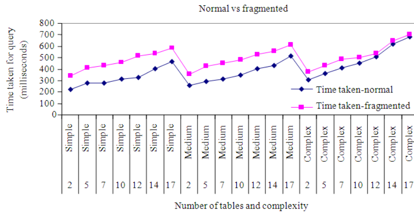
Fig 2: Performance between normal and fragmented environment
