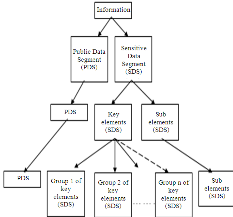
Fig. 1: Data fragmentation
