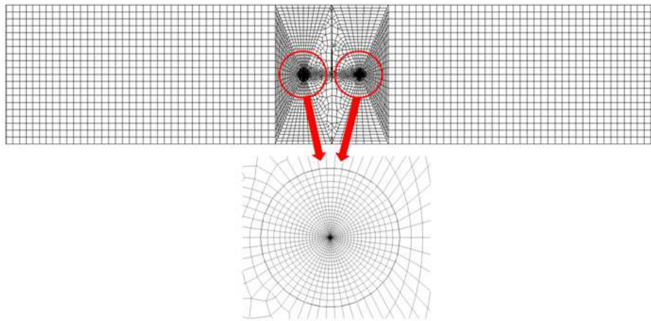
Fig. 2. Typical finite element mesh pattern of the bi-material four point bend specimen
