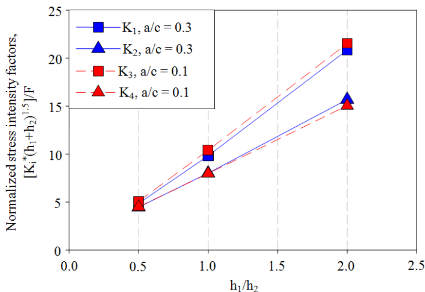
Fig. 4. Variation of the normalized stress intensity factors versus h_1/h_2 ratio
