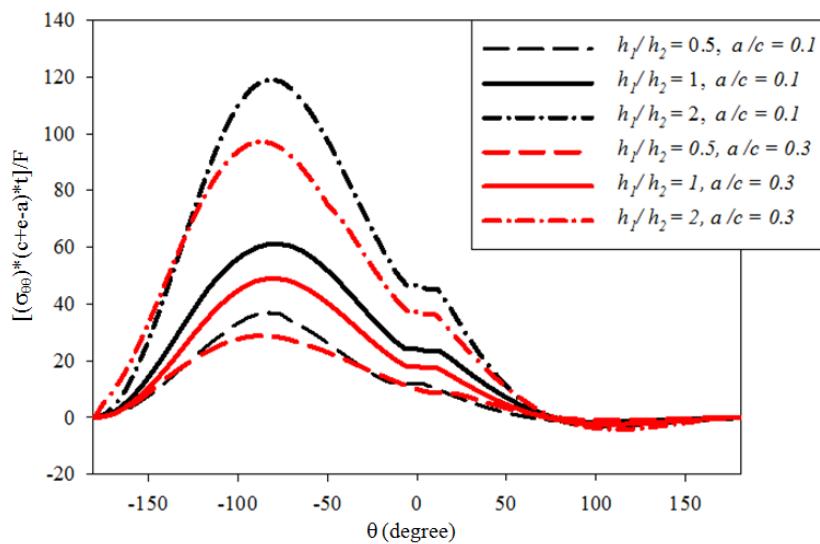
Fig. 3. Distribution of the normalized tangential stress versus tangential direction at r = r_c = 0.2 mm
