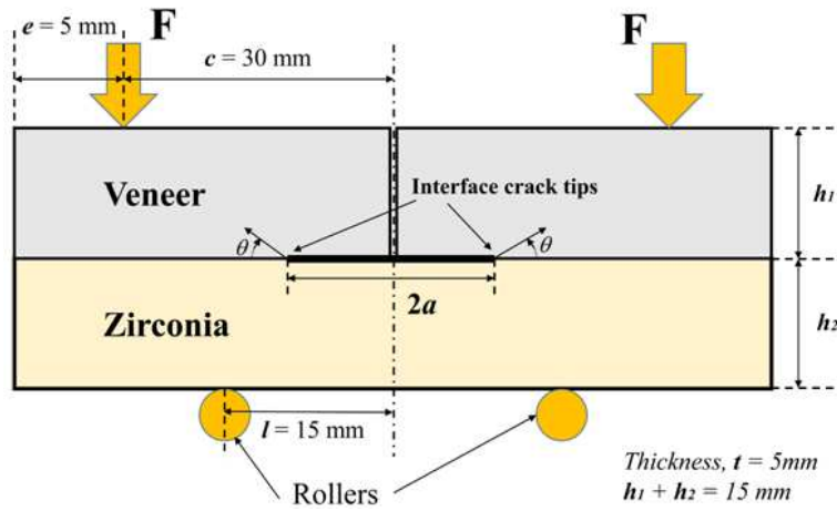
Fig. 1. General configuration of the bi-material four point bend specimen
