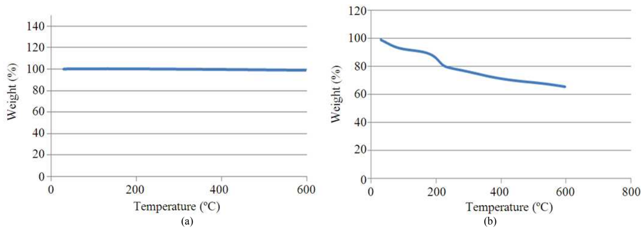
Fig. 2. TGA patterns of graphite powder (A) and GO (B)
