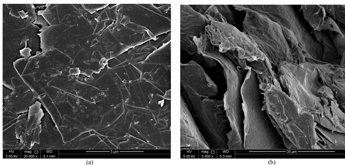
Fig. 4. SEM images of graphite powder (A) and GO (B) before incubation with the microorganisms
