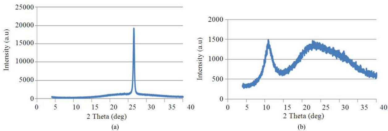
Fig. 1. XRD Patterns of graphite (A) and GO (B)
