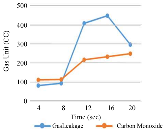
Fig. 3: Gas reading for MQ5 and MQ7
