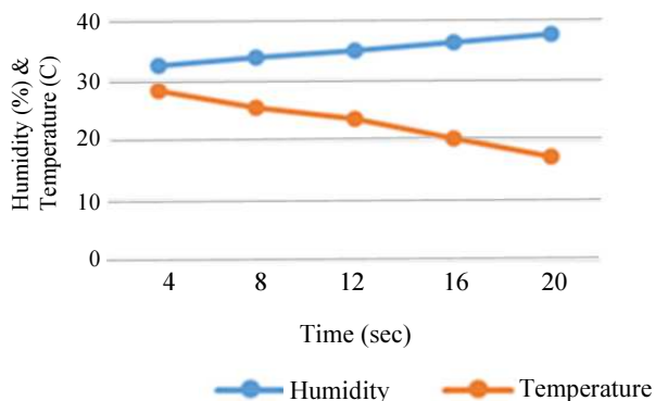
Fig. 2: Humidity and temperature of DHT11
