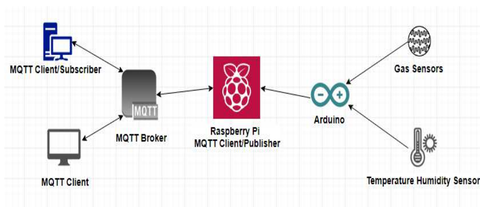
Fig. 1: Proposed Architecture for IOT Based GHMS
