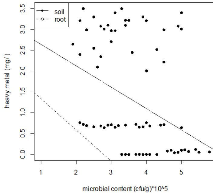
Fig. 4. Correlation between heavy metal and microbial content in soil and root in mangrove forest ( R. racemosa ) in the Niger River Delta, Nigeria. It indicates a negative relationship, as heavy metal increases the microbial content decreases
