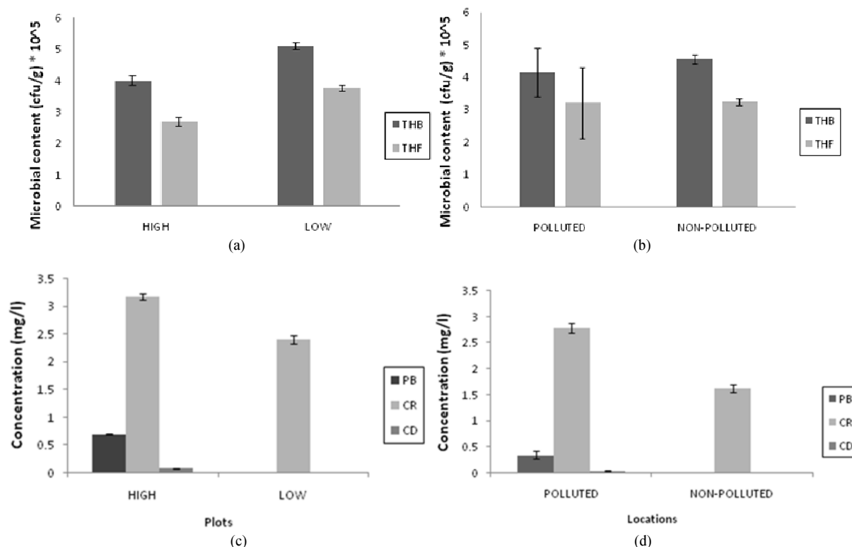
Fig. 2. Graphs of microbial and heavy metal concentrations in mangrove soil: (a) Microbial content in highly and lowly polluted plots (b) Polluted and non-polluted locations; and heavy metal concentrations in (c) Highly and lowly polluted plots; (d) Polluted and non-polluted locations in the Niger Delta, Nigeria. THB = Total Heterotrophic Bacteria and THF = Total Heterotrophic Fungi. Vertical lines show \pm 1 standard error of the mean
