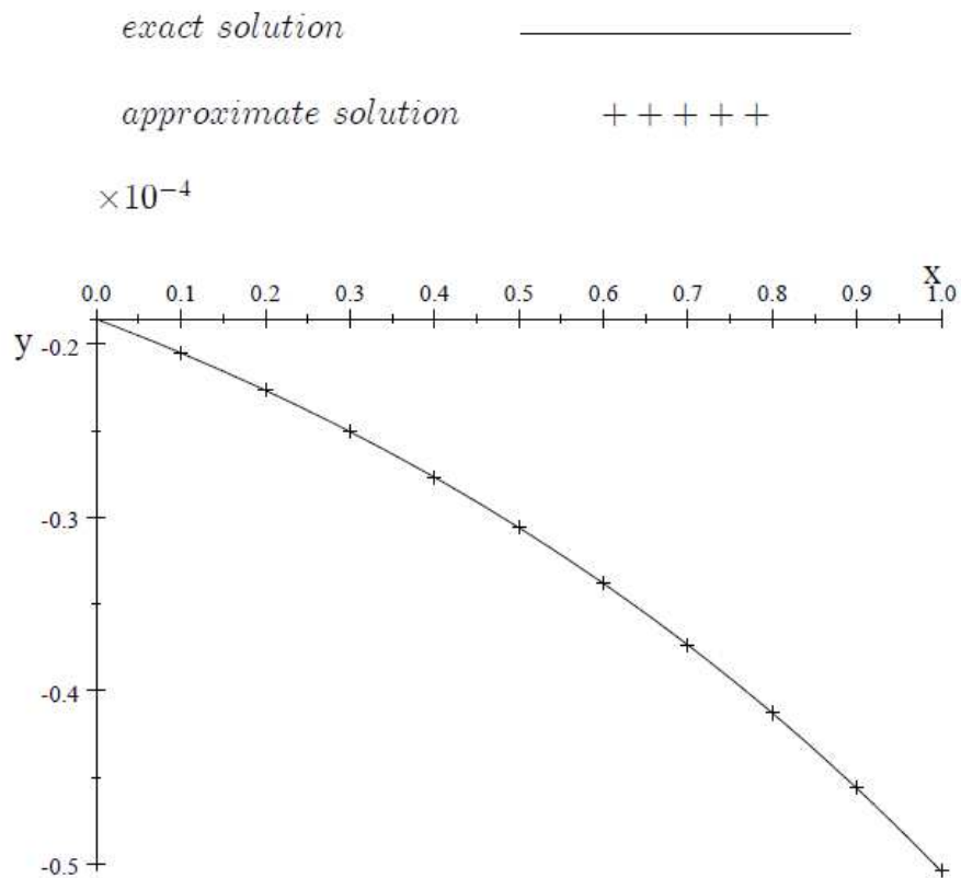
Fig. 2. Exact and approximate solutions for ( n = 5 ) of example (4.2)
