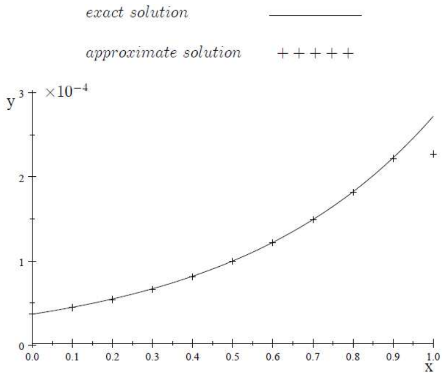
Fig. 1. Exact and approximate solution ( n = 4 ) of example (4.1)
