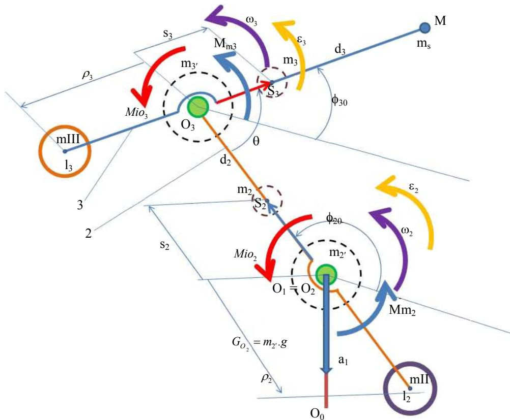
Fig. 4: Dynamics of balanced plan cinematic chain
