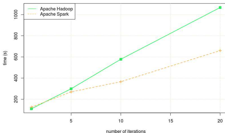
Fig. 5. Running time of Spark/Hadoop with different number of iterations on 360*360*360 points computational domain
