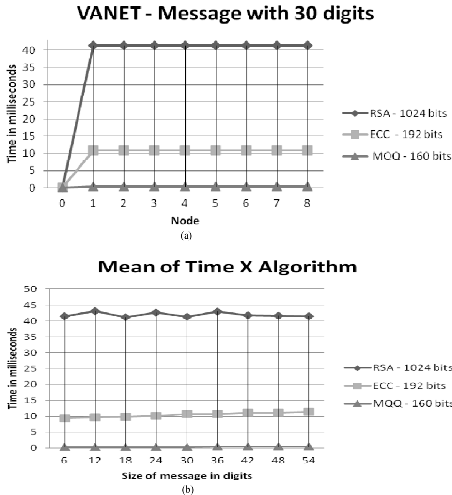
Fig. 8. Comparison of RSA, ECC and MQQ with compatible keys
