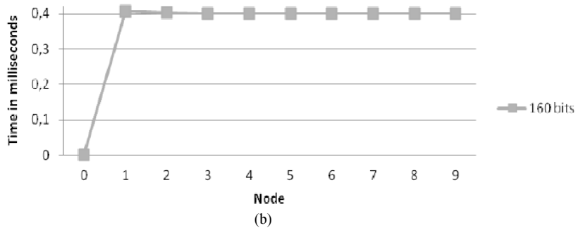
Fig. 5. Time of a communication in Vanet with ECC and MQQ
