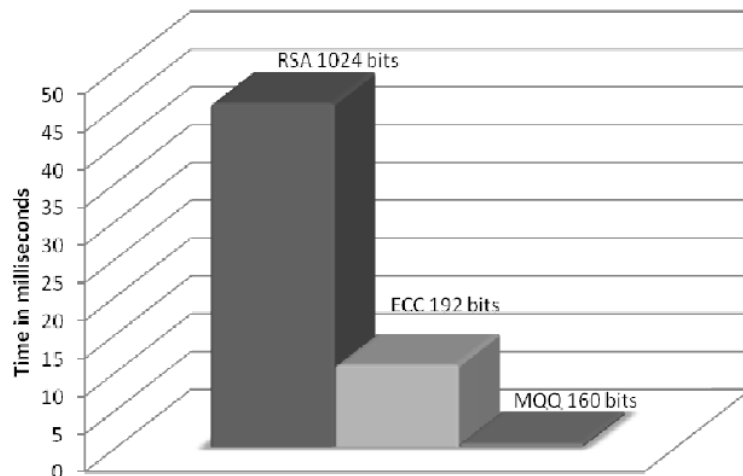
Fig. 2. Execution Time of the Algorithms RSA, ECC and MQQ on a desktop
