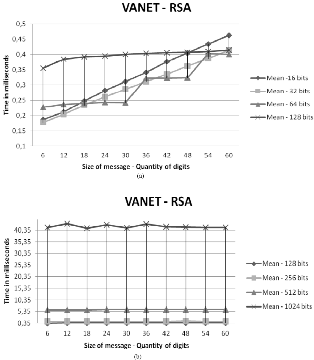
Fig. 6. Mean time using RSA, (a) keys to 128 (b) from 128 to 1K
