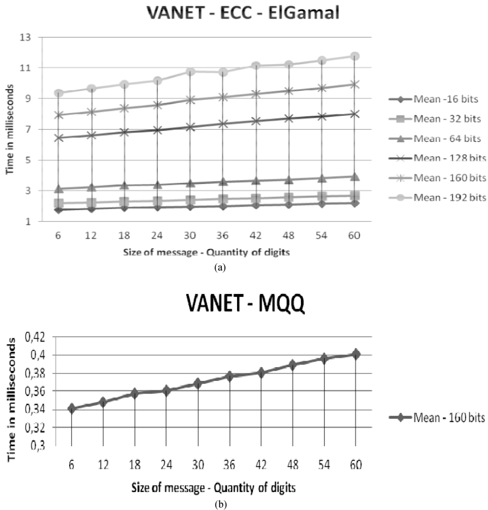
Fig. 7. Execution time using ECC and MQQ
