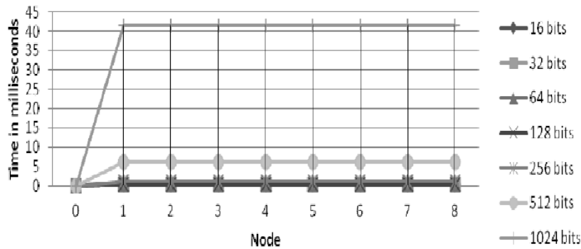
Fig. 4. Time of a communication in Vanet with RSA
