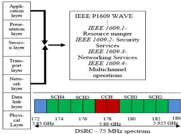
Fig. 1. IEEE WAVE and DSRC (Yanamandram, 2009)
