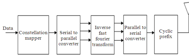
Fig. 3. OFDMA transmitter
