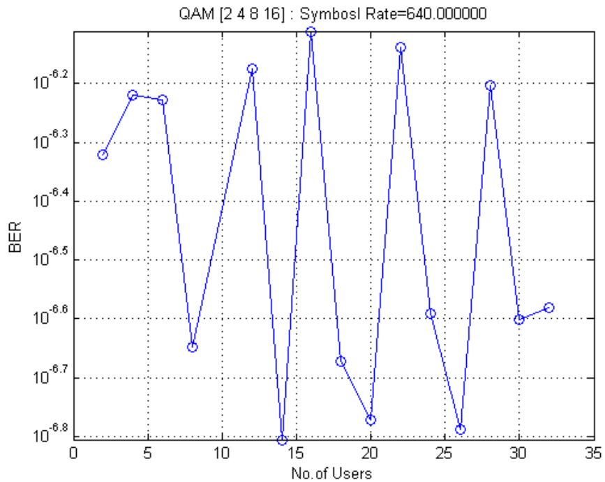
Fig. 12. MC-CDMA System M-ary QAM
