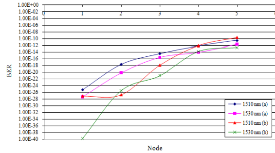
Fig. 6: BER performance at each node in ring network for working channels \lambda(a) and protection channel \lambda(b) for a wavelength of 1510 nm and 1530 nm
