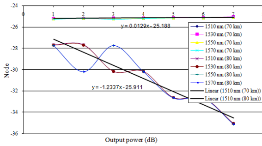
Fig. 17: Comparison of output power at distance between two nodes (70 km and 80 km); where the value of gain amplifier has been prescribed. The value of amplifier gain is equal to load line for a distance between two nodes is 70 km.
