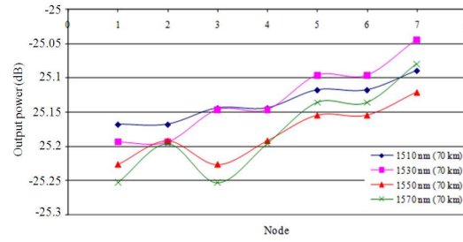
Fig. 15: Output power for each node in metropolitan mesh network; where the distance between two nodes is 70 km
