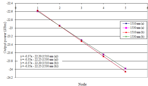
Fig. 5: Output power at each node in ring network for working channels \lambda(a) and protection channel \lambda(b) for a wavelength of 1510 nm and 1530 nm
