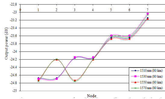
Fig. 19: Output power for each node in metropolitan mesh network; where the distance between two nodes is 80 km.
