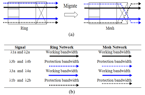
Fig. 3: (a) Migration topology use a configuration of OXADM 2 and (b) Function of bandwidth for both topologies
