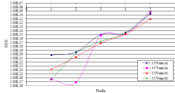
Fig. 8: BER performance at each node in ring network for working channels \lambda(a) and protection channel \lambda(b) for a wavelength of 1550 nm and 1570 nm
