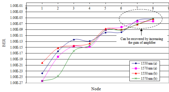
Fig. 10: BER of each node for mesh network on working channel
