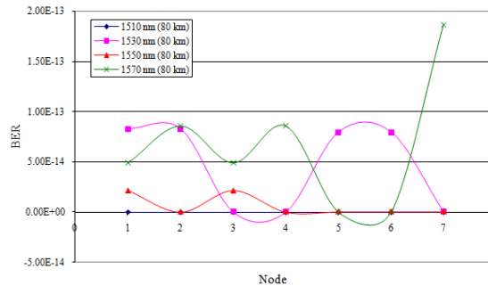
Fig. 20: BER performance for each node in metropolitan mesh network; where the distance between two nodes is 80 km
