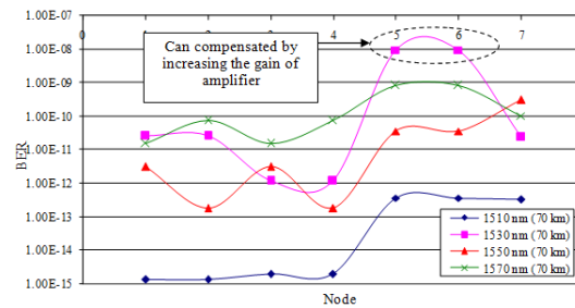
Fig. 16: BER performance for each node in metropolitan mesh network; where the distance between two nodes is 70 km
