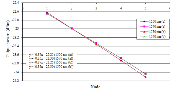
Fig. 7: Output power at each node in ring network for working channels \lambda(a) and protection channel \lambda(b) for a wavelength of 1550 nm and 1570 nm.
