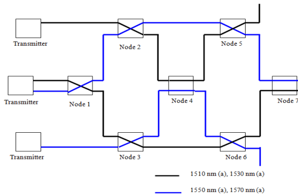
Fig. 14: Signal propagation paths in mesh network using configuration OXADM 2 as a distribution node. The next simulation study will refer to these signal paths
