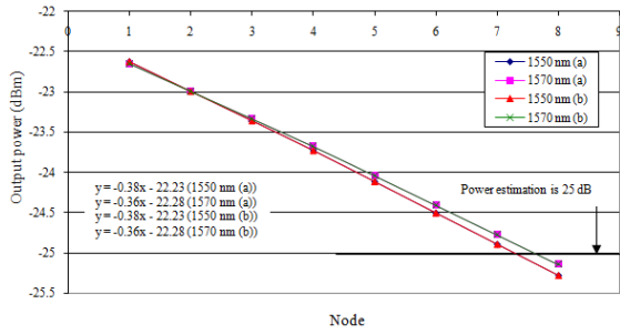
Fig. 9: Output power of each node for mesh network on working channel
