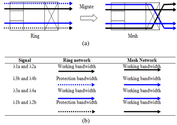
Fig. 2: (a) Migration topology use a configuration of OXADM and (b) Function of bandwidth for both topologies
