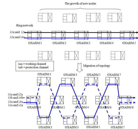
Fig. 4: Migration of topology from ring to mesh using OXADM 1 configuration. OXADM handle half of transmission capacity for ring network and using full of transmission capacity for mesh networks
