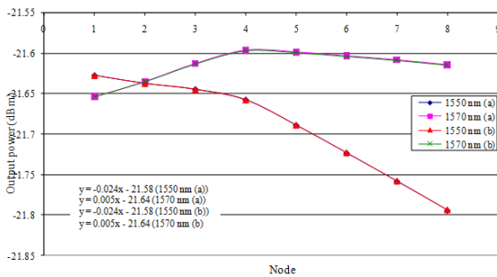
Fig. 11: The increasing of preamplifier gain at 0.36 dB will keep the constant value of output power at each node in mesh network (working channel)
