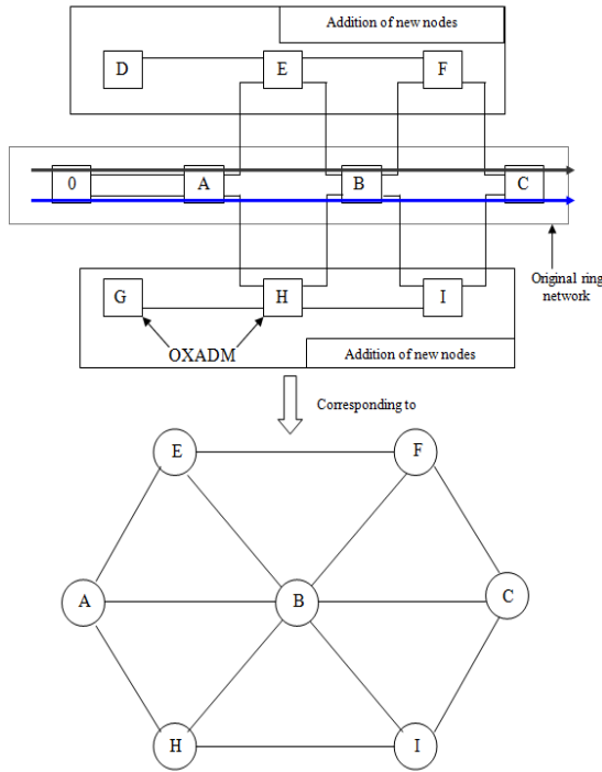
Fig. 13: Migration of topology from ring to mesh network using OXADM2 configuration. OXADM used only half transmission capacity on ring network and mesh network
