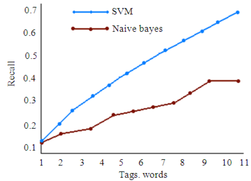
Fig. 2: Recall
