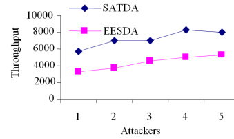
Fig. 7: Attackers Vs throughput we can see that throughput of our proposed SATDA protocol is higher than the existing EESDA protocol
