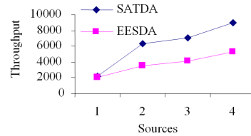
Fig. 12: Sources Vs throughput we can see that throughput of our proposed SATDA protocol is higher than the existing EESDA protocol
