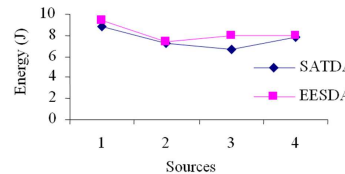
Fig. 10: Sources Vs energy we can see that the Energy consumption of our proposed SATDA protocol is less than the existing EESDA protocol
