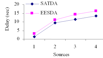
Fig. 8: Sources Vs delay we can see that the average end-to-end delay of our proposed SATDA protocol is less than the existing EESDA protocol
