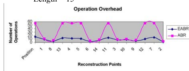
Fig. 29: Operation Overhead: Network = 40, Route Length = 15
