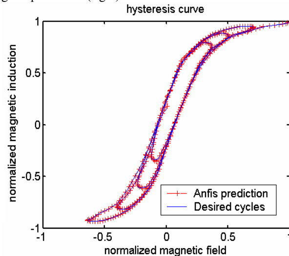
Fig. 8 : Hysteresis curves
