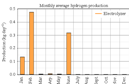
Fig. 19: Monthly hydrogen production for the grid connected PV-wind-hydrogen system
