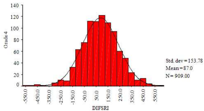
Fig. 4: Histogram of grade 4 SRI lexile difference scores
