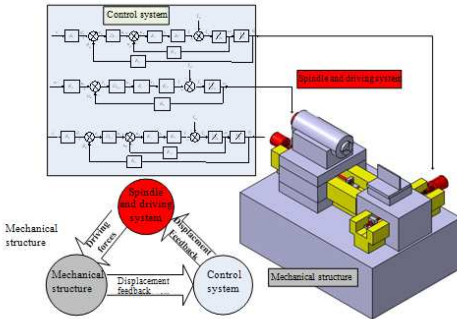
Fig. 1: A typical precision machine tool integrated model
