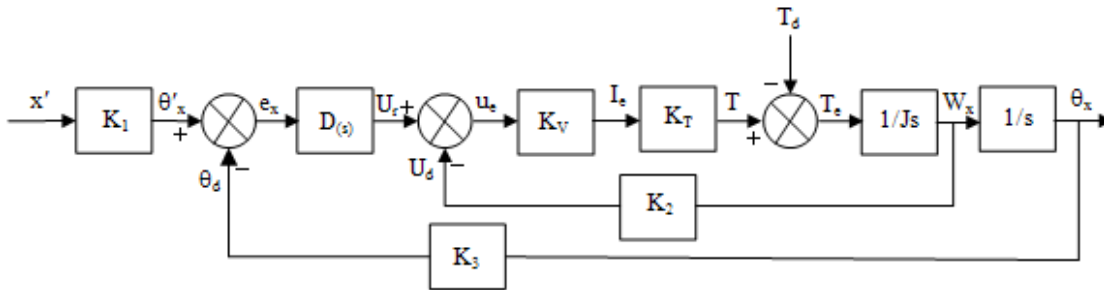
Fig. 3: Dynamic model of slide control system
