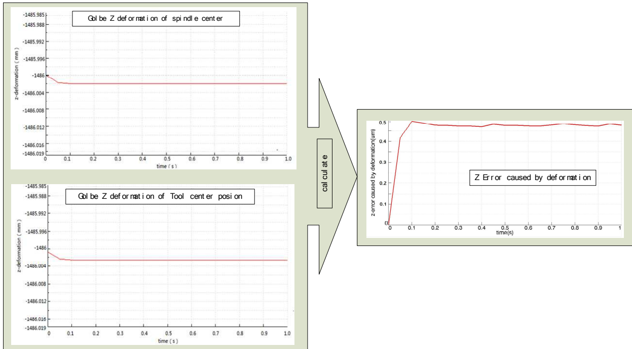
Fig. 7: Globe deformation in Z direction between tool center position and spindle center
