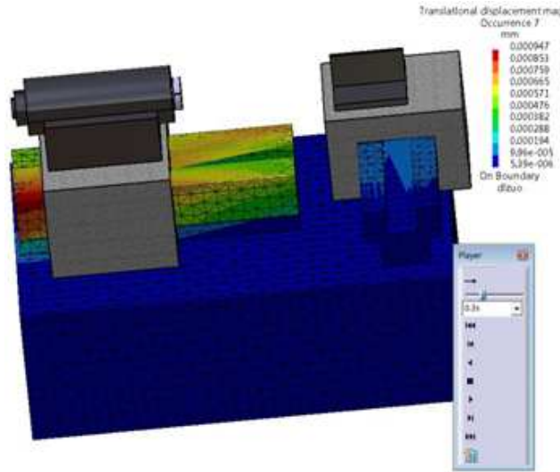
Fig. 5: Screenshot of the virtual machine tool in analysis
