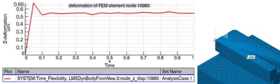
Fig. 6: Deformation in motion of a point on fixed slide way
