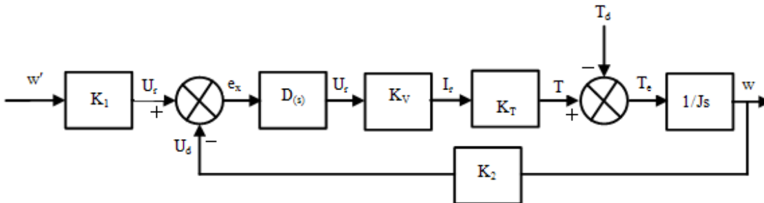
Fig. 4: Dynamic model of spindle control system
