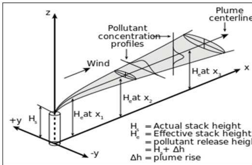
Fig. 2. Gaussian distributions in the horizontal and vertical directions (Source: Masters, 1977)
