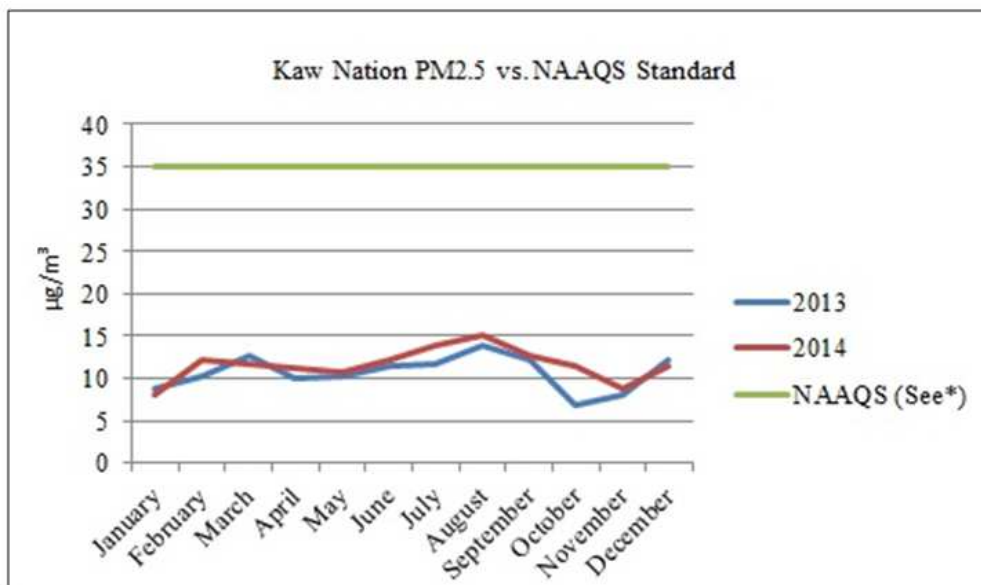
Fig. 8. Kaw Nation Monthly PM2.5 (Source: Kaw Nation); *NAAQS Standard for PM2.5: A 24 h average not to exceed 35 µg/m 3 ; **Months are reported in Monthly Mean
