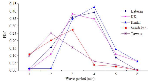
Fig. 3: Probability distribution of wave periods
