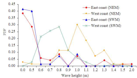
Fig. 4: Probability distribution of wave height according to area and monsoonal seasons
