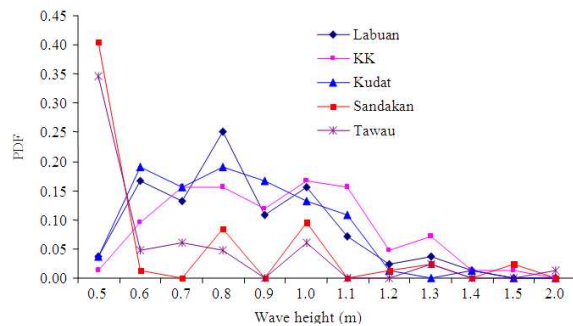
Fig. 2: Probability distributions of wave heights
