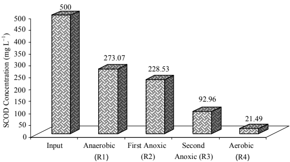
Fig. 3: The average effluent soluble COD concentration from each reactor during experiment
