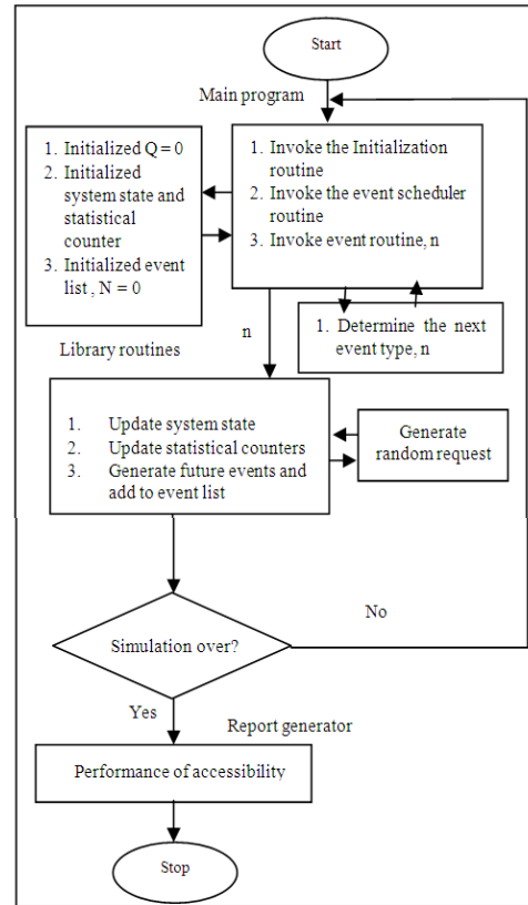
Fig. 2: Flow of the simulator
