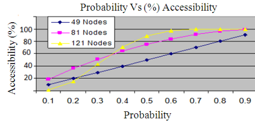
Fig. 4: Percentage of accessibility result
