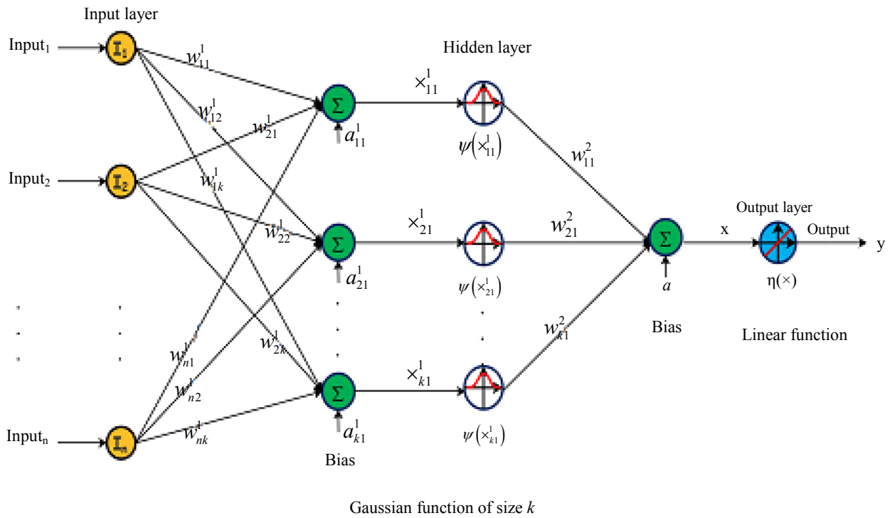
Fig. 2: The RBF architectural model
