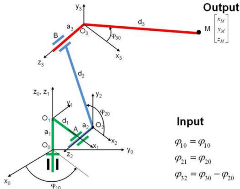
Fig. 1. Geometry and direct kinematics to a MP-3R
