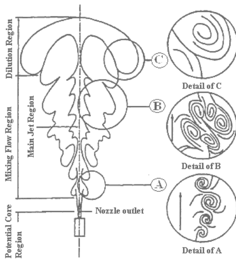
Fig. 1: Transient gaseous jet structure [33]
