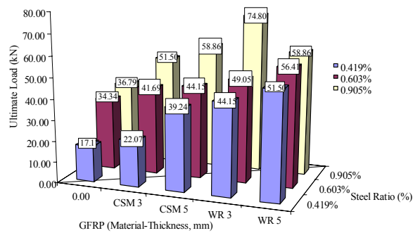
Fig. 5: Ultimate load
