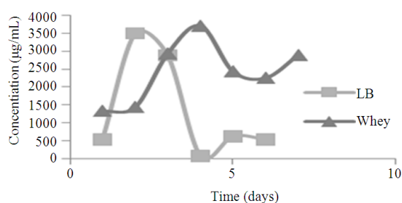
Fig. 2. Comparison of lactic acid production by isolate 12a in Luria Bertani and whey water
