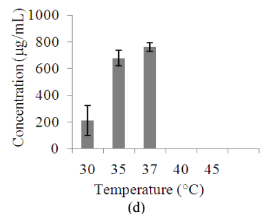
Fig. 1. Lactic acid production by bacterial isolates. (a) Lactic acid production in LB after 24 h of growth by the 15 LAB isolates namely 1b, 3b, 4b, 5b, 6b, 7b, 9b, 10a, 11b, 12a, 13b, 14, 15b, 16, 17 as per the source of isolation mentioned in the materials and method; (b) Screening of Lactic acid production by 16 selected strains (1b, 3b, 4b, 5b, 6b, 7b, 9b, 10a, 10b, 11b, 12a, 13b, 14, 15b, 16, 17) in whey water after 36 h of growth; (c) Effect of pH on lactic acid production by isolate 12a in whey water after 12 h of growth; (d) Effect of Temperature on lactic acid production by isolate 12a in whey water after 12 h of growth
