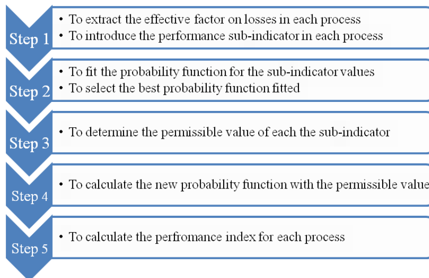
Fig. 2: The proposed method algorithm
