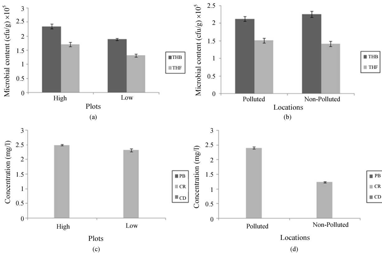
Fig. 3: Graphs of microbial and heavy metal concentrations in mangrove root: (a) Microbial content in highly and lowly polluted plots (b) Polluted and non-polluted locations; and heavy metal concentrations in (c) Highly and lowly polluted plots; (d) Polluted and non-polluted locations in the Niger Delta, Nigeria. THB = Total Heterotrophic Bacteria and THF = Total Heterotrophic Fungi. Vertical lines show \pm 1 standard error of the mean
