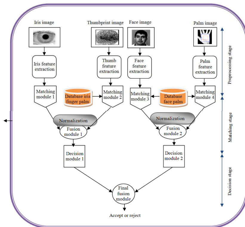
Fig. 2. A framework of the proposed score/ decision-level fusion
