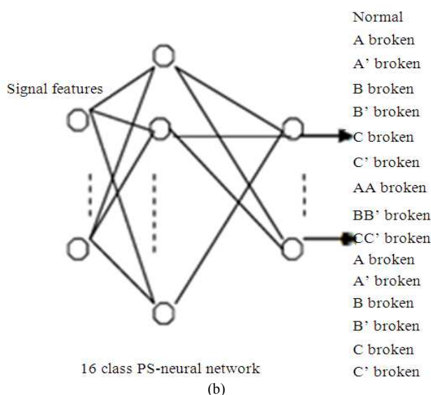
Fig. 8. Two architectures of PS-neural network systems for classifying multiple classes of faults in a three-phase electric drive, (a) A structured PS-neural network system, (b) A single multi-class PS-neural network system
