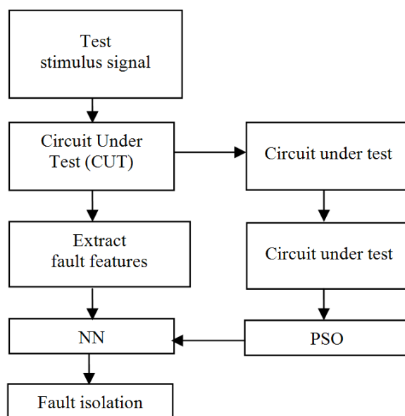
Fig. 2. Flow chart of PSO neural network fault diagnosis
