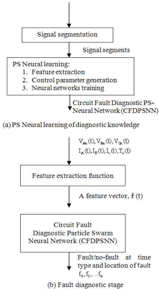
Fig. 4. A multi-class PS neural network for circuit fault diagnosis
