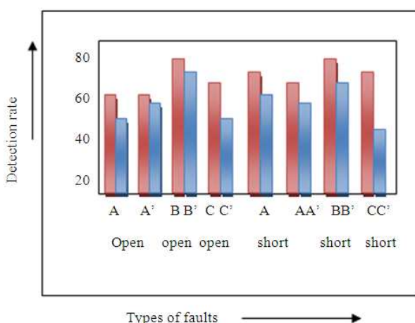
Fig. 10. Performances of the two PS neural networks
