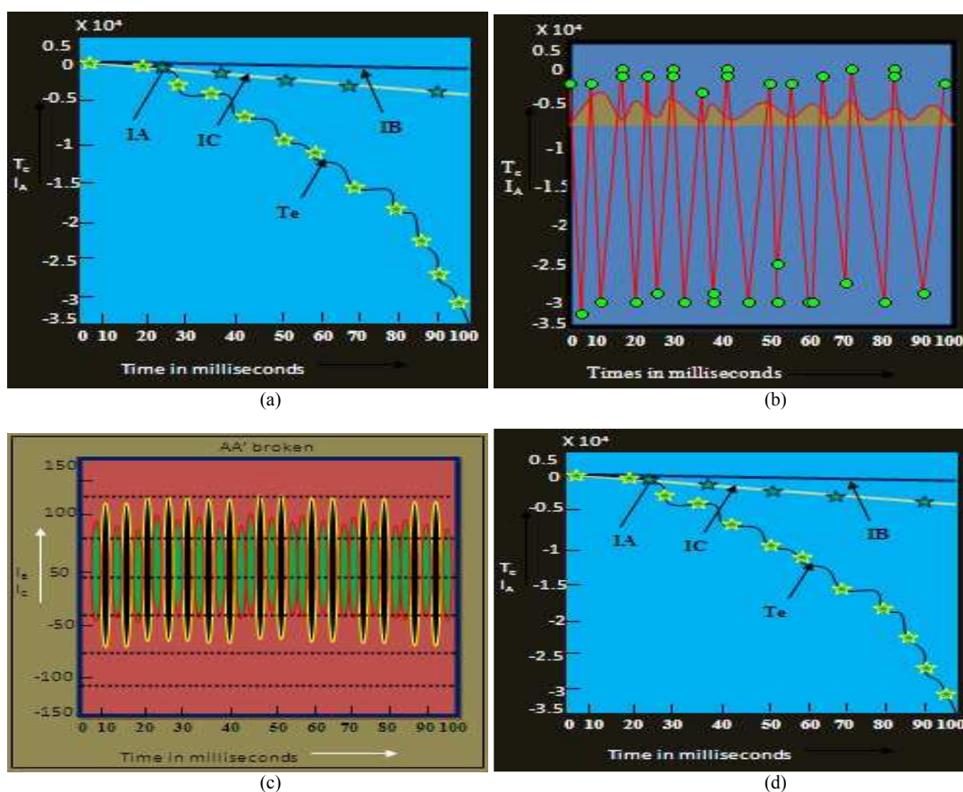
Fig. 3. Plots showing currents, I_A , I_B , I_C and Torque T_e under various fault conditions at operating point: torque=100 nm, speed=600 rpm. Time is in msec. (a) Signals I_A (in Blue), I_B (in Red), I_C (in green) and T_e (in black) when switch A is open, (b) Signals I_A (in blue) and T_e (in red) when switches AA' are broken, (c) Signals I_B (in blue) and I_C (in red) when Switches AA' are broken, (d) Signal I_A (in blue), I_B (in red), I_C (in green) and T_e (in black) when Switch A is shorted
