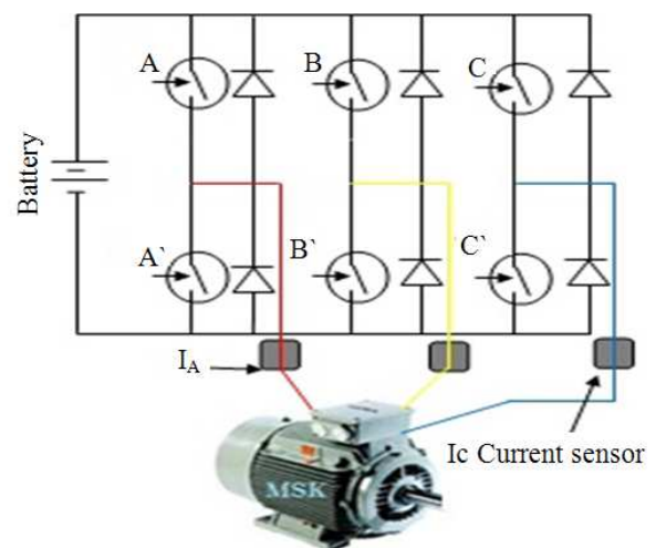
Fig. 1. A six-switch inverter in a three-phase electric drive model
