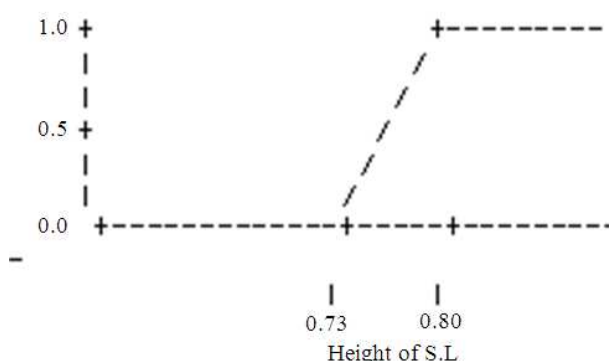
Fig. 1. Shows the Fuzzy values for sepal length
