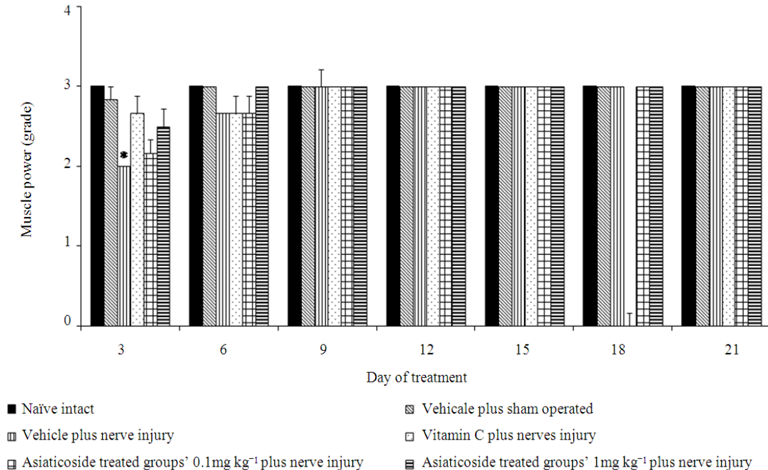
Fig. 3. The effect of asiaticoside on the recovery of motor function of sciatic nerve was assessed using muscle power. Data are present as mean \pm SEM (n = 6 group -1 ) * p-value < .05 all; compared with the vehicle plus sham treated group
