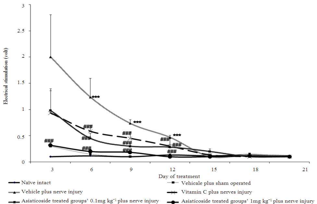
Fig. 5. The effect of asiaticoside on the recovery of motor function of sciatic nerve was assessed using foot withdrawal reflex in response to pain induced by electrical stimuli. Data are present as mean \pm SEM ( n = 6 group -1 ) *** p -value < .001 all; compared between vehicle plus sham treated group and all groups which receive crush injury, ### p < 0.001 all; compared between vehicle plus crush injury
