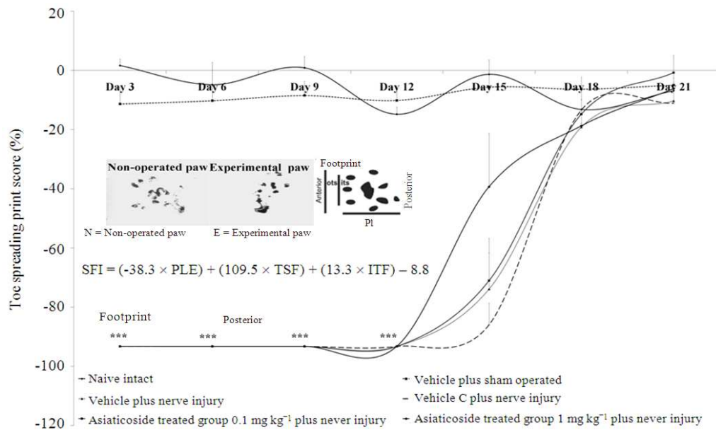
Fig. 4. The effect of asiaticoside on the recovery of motor function of sciatic nerve was assessed using the Sciatic nerve Function Index (SFI) or toe spreading score. Data are present as mean \pm SEM ( n = 6 group -1 ) p < 0.001 all; compared between vehicle plus sham treated group and all groups which receive crush injury
