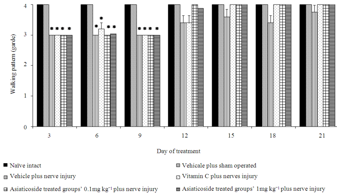
Fig. 2. The effect of asiaticoside on the recovery of motor function of sciatic nerve was assessed using walking pattern analysis. Data are present as mean \pm SEM (n = 6 group -1 ) * p-value < .05 all; compared with the vehicle plus sham treated group
