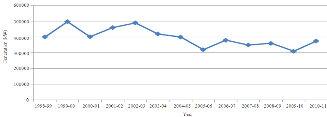
Fig. 2: Muppandal-225kW wind turbines generation details for the period of 1998-2011
