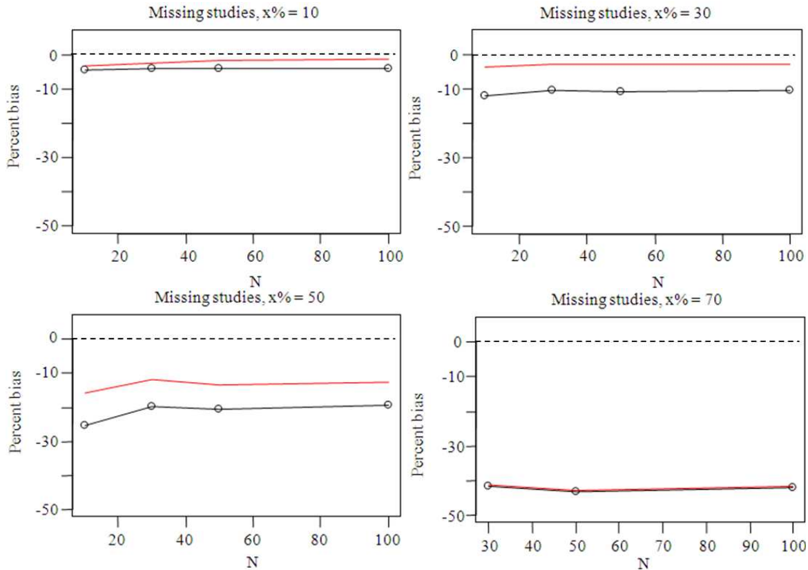
Fig. 1: Percentage relative bias for different levels of missing publications. Note: Red line: Percentage relative bias after the application of Trim and Fill method; Black line: Percentage relative bias with X% studies missing
