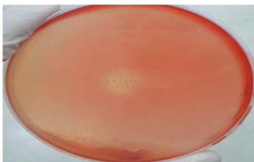
Fig. 4: Clear zone indicated the hydrolysis of CMC as a result of cellulases production by isolated Geobacillus pallidus
