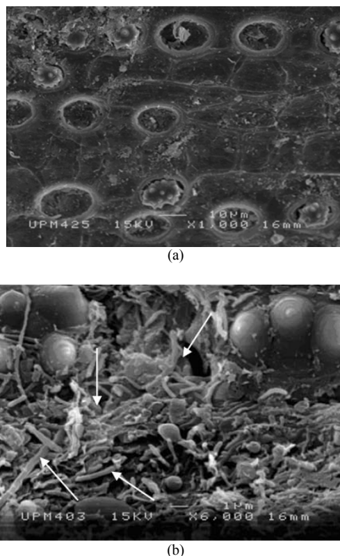
Fig. 1: SEM observation on the EFB compost sample at day 7 treatment (a): 1000X magnification and (b): 6000X magnification. The arrows showed the colonization of bacteria
