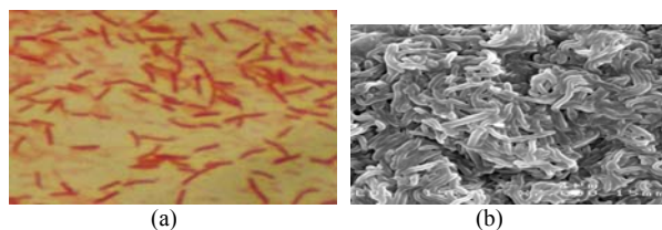
Fig. 3: Gram stain result viewed under 1000x light microscope (a) and scanning electron microscope micrograph of isolated bacteria under 7000x (b)
