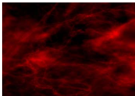
Fig. 6: FISH staining on pure culture of thermophilic cellulase-producing bacteria isolated from EFB-POME compost
