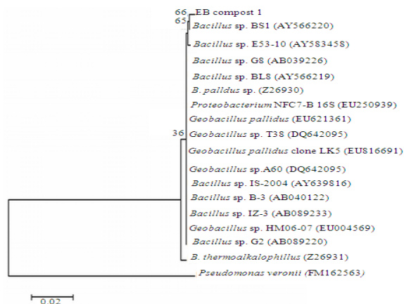
Fig. 5: Neighbor joining phylogenetic trees. The trees were generated using the 17 alignments matches
