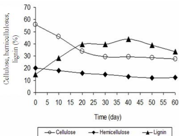
Fig. 2: The profiles of cellulose (○): Hemicellulose (◆) and lignin content (▲) of EFB-POME compost sample throughout the treatment
