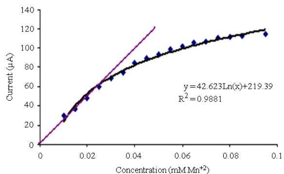
Fig. 5a: Plot of oxidation current versus different concentration 0.01-0.1 mM MnCl 2 in blood sample at scan rate 100 mV sec -1 using CNT/GCE versus Ag/AgCl
