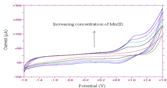
Fig. 4: Cyclic voltammogram for the redox peaks of Mn 2+ (different concentration 0.1-3 mM) in blood sample at scanning rate 100 mv sec -1 using CNT/GCE versus Ag/AgCl
