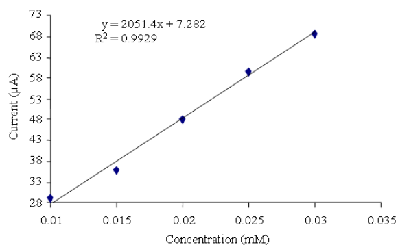
Fig. 5b: Plot of oxidation current versus different concentration 0.01-0.03 mM MnCl 2 in blood sample at scan rate 100 mV sec -1 using CNT/GCE versus Ag/AgCl
