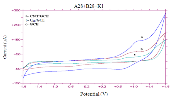
Fig. 3: Cyclic voltammogram of 0.5 mM Mn 2+ in blood sample as supporting electrolyte at scanning rate 100 mV sec -1 using (a) CNT/GCE (b) C 60 /GCE and (c) GCE versus Ag/AgCl
