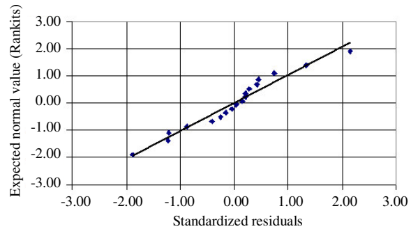
Fig. 2: Model adequacy checking (expected normal value vs. standardized residuals)
