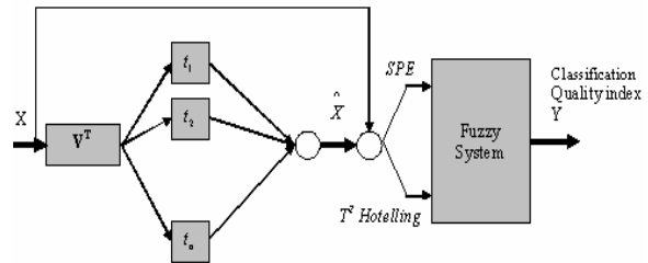
Fig.2: Principle of Quality Classification Using PCA-Fuzzy System
