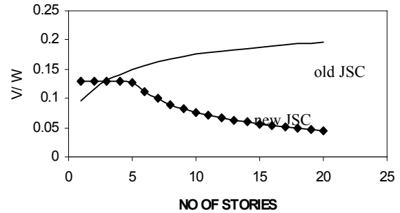
Fig. 3: Number of stories versus V/W
