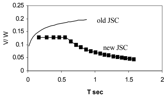
Fig. 2: Period of structure in sec versus V/W
