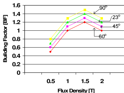
Fig. 5: Building factor for each T-joint
