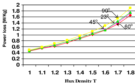
Fig. 4: Graph of power loss from measurement
