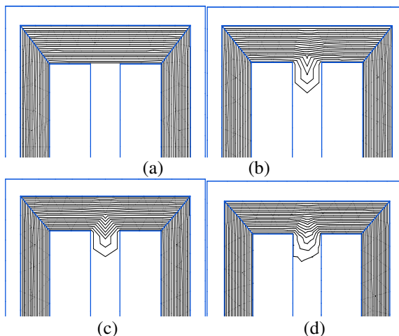
Fig. 6: Variation of magnetic flux lines in transformer core built M5 material use Software with \omega t=0 (a) T- joint 90°, (b) T-joint 23°, (c) T- joint 45° and (d) T-joint 60°
