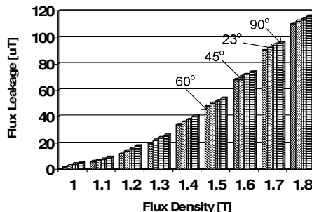
Fig. 7: Flux leakages at T-joint
