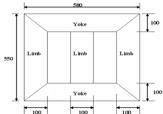
Fig. 2: Dimension (mm) of 100kVA transformer model
