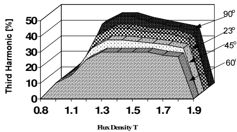
Fig. 8: Harmonic analysis of third component distortion
