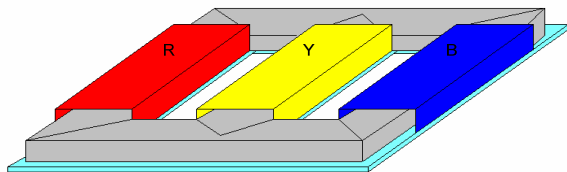
Fig. 3: 100kVA Transformer Model with 45° T-Joint
