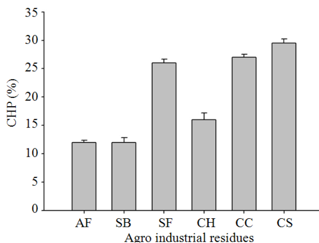
Fig. 2. Critical humidity point of the agro industrial residues: Agave Fibers (AF), Sugarcane Bagasse (SB), Sotol Fibers (SF), Coconut Husk (CH), Corn Cobs (CC) and Candelilla Stalks (CS)
