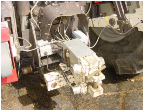
Fig. 2: The draw bar dynamometer used for measuring draft
