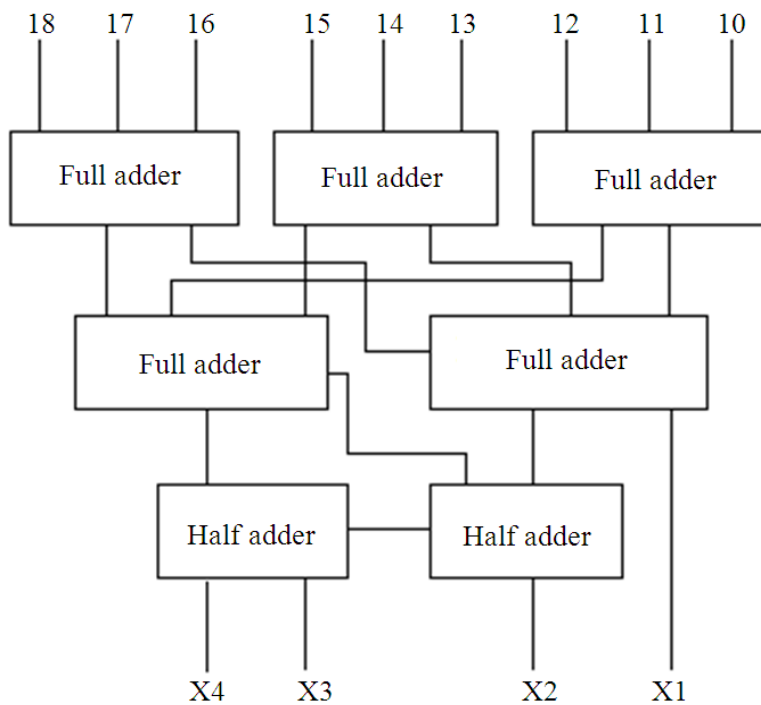
Fig. 2. 9-4 Compressor design
